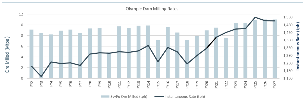
Figure 2: Processing historical milling rates compared to SDP target rates from FY23 – FY25
