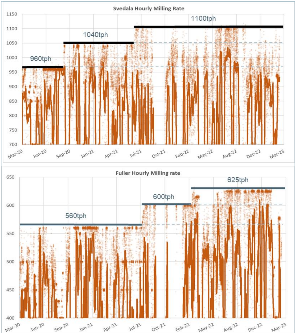
Figure 3: Incremental improvement of milling rates
