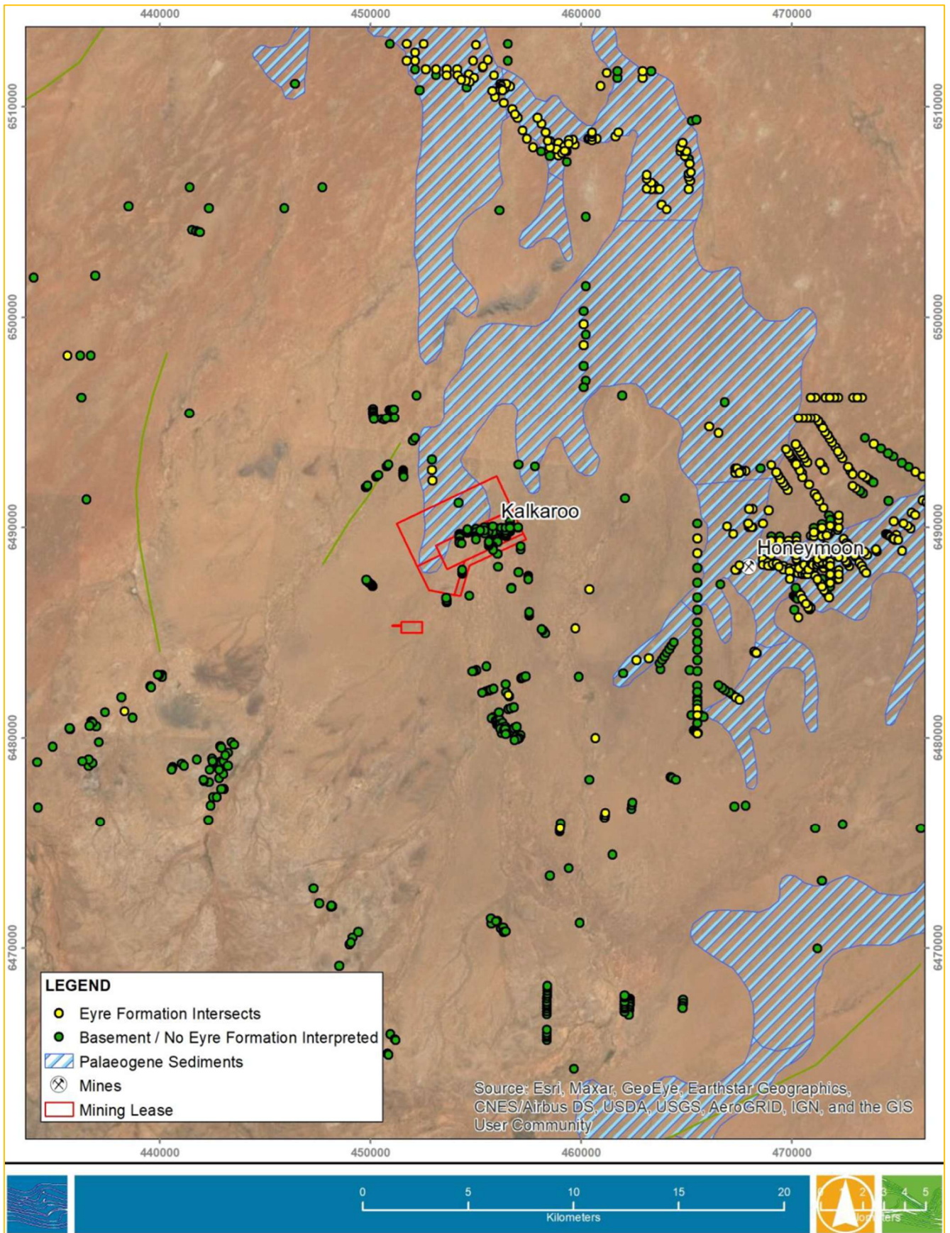
Figure 10: Tertiary (Palaeogene) Sedimentary Distribution (SARIG).
