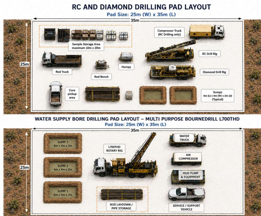
Plate 6. Typical drill pad layouts
