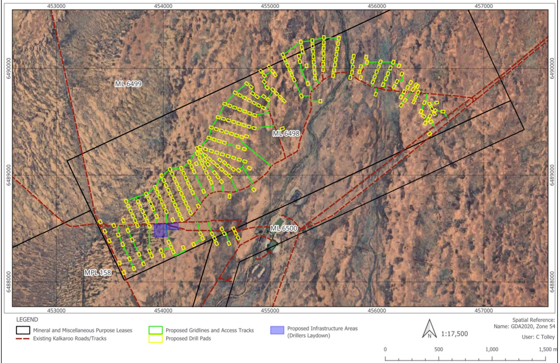
Figure 4: Location of proposed resource drill collars, access tracks, and laydown area
