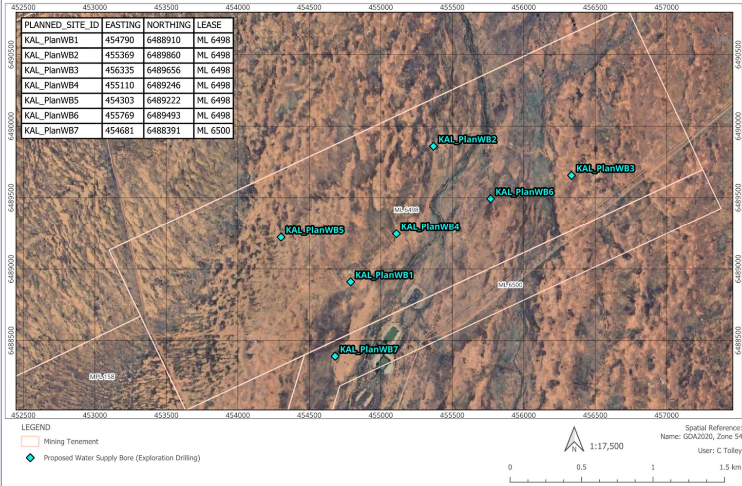
Figure 9: Proposed Groundwater Supply Bore Location Plan
