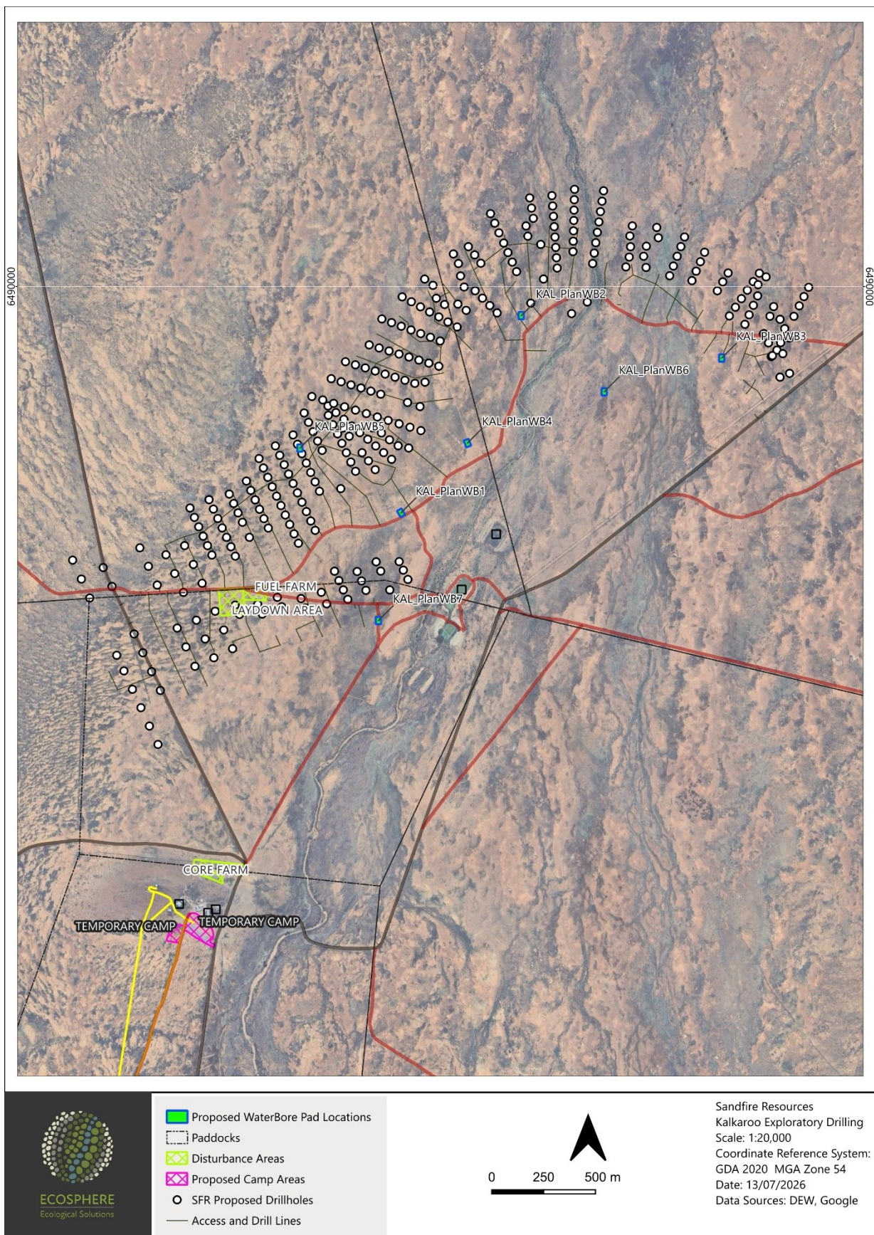
Figure 4. Planned drill holes on previously rehabilitated area.
