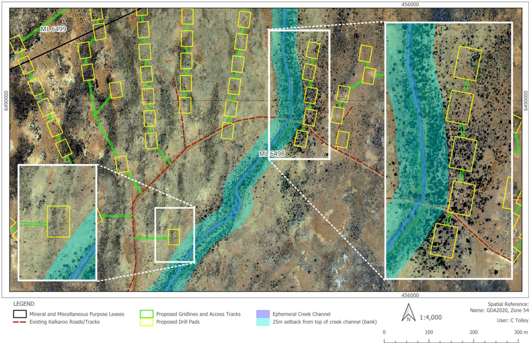
Figure 5: Location of proposed resource drill collars, access tracks, over aerial image in relation to ephemeral watercourse.
