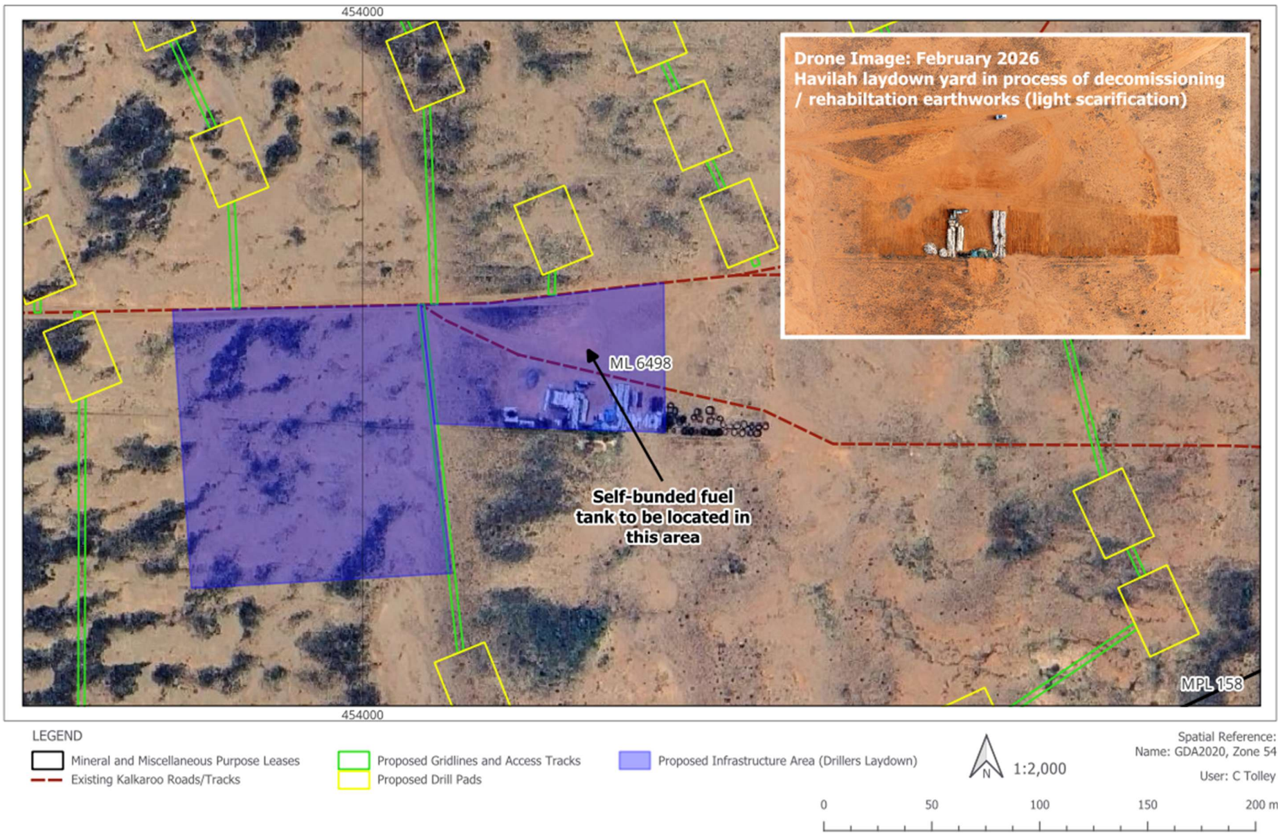
Figure 8: Proposed Drillers Laydown Yard
